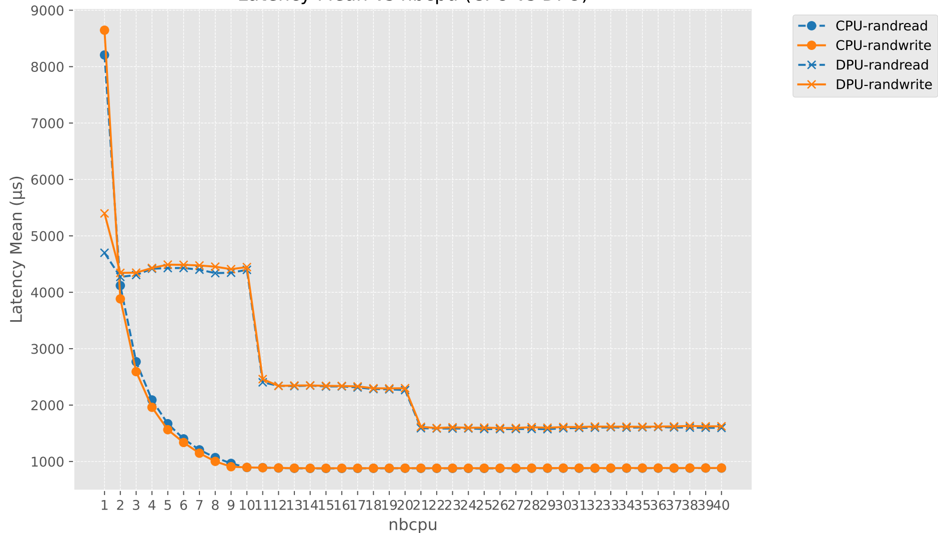
Latency Mean vs nbcpu (CPU vs DPU)
